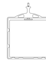
Filter Frame Combo 5.65"x5.65"/4"x5.65" vertical, K2.65148.0
