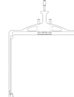
Filter Frame Combo 5.65"x5.65"/5"x6" horizontal, K2.65022.0
