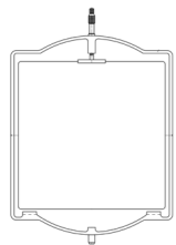
Filter Frame 6.6"x6.6" non geared for SMB-1, MB-14, K4.47074.0
